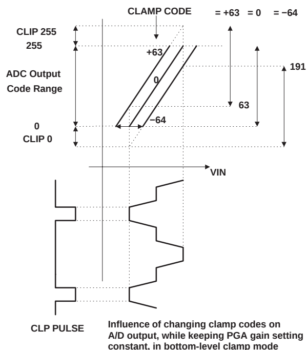
Figure 2-2. Bottom-Level Clamping
